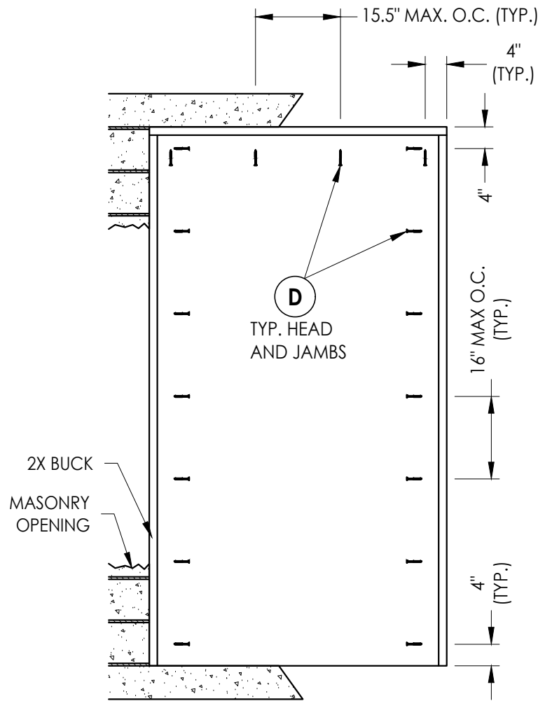
BUCK ANCHORING
