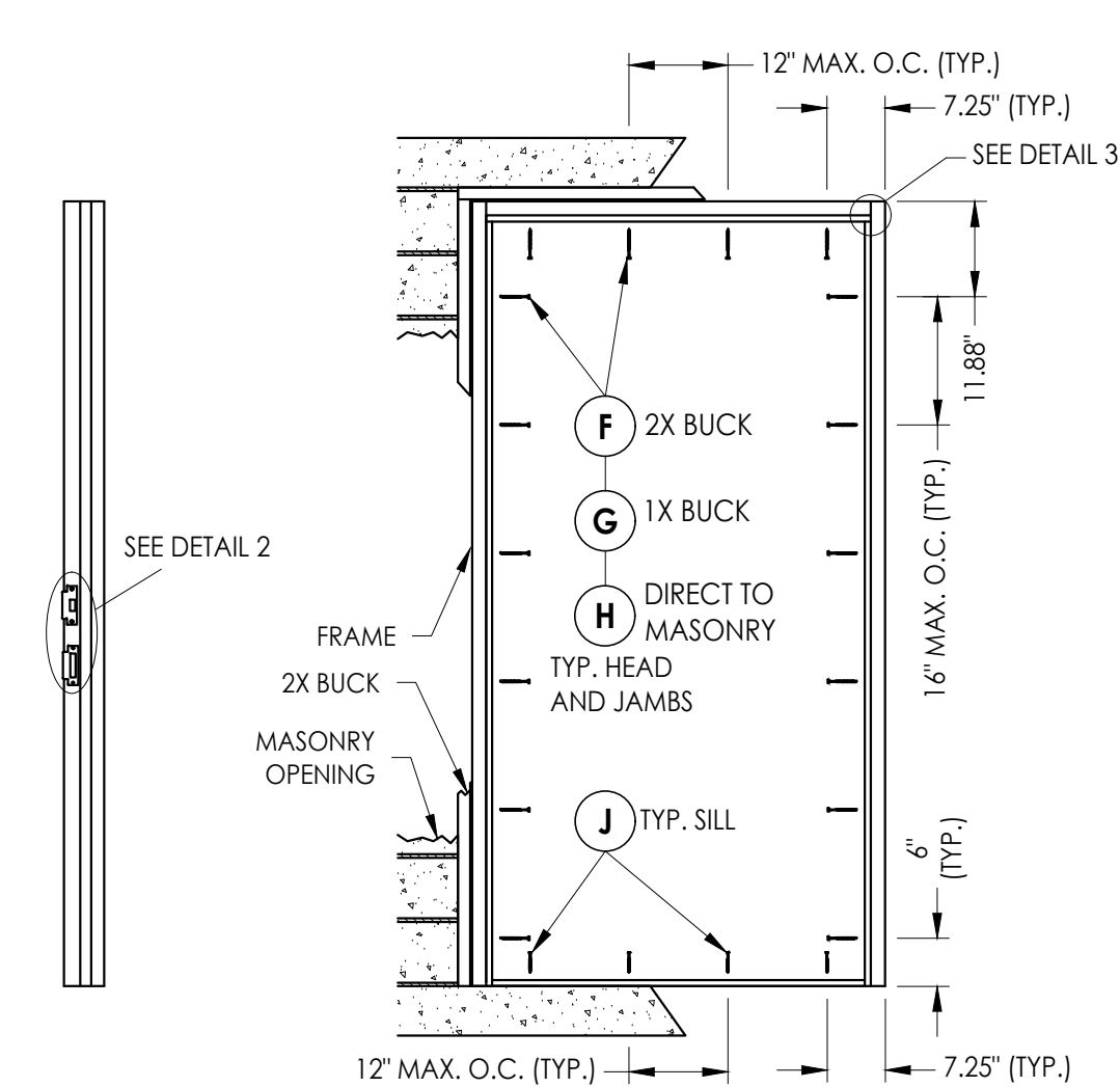
FRAME ANCHORING
